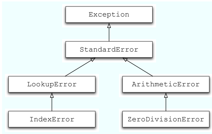
Figure 12.3: Exception hierarchy
