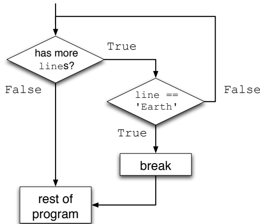
Figure 7.10: The break statement
