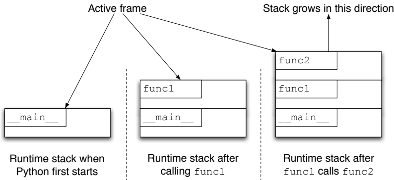
Figure 7.8: Runtime stack
